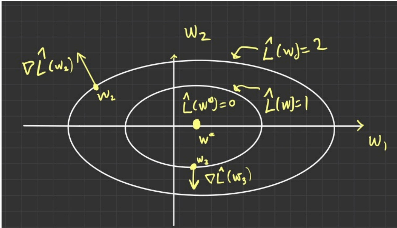
FIGURE 1. Illustration of the gradient of the loss
