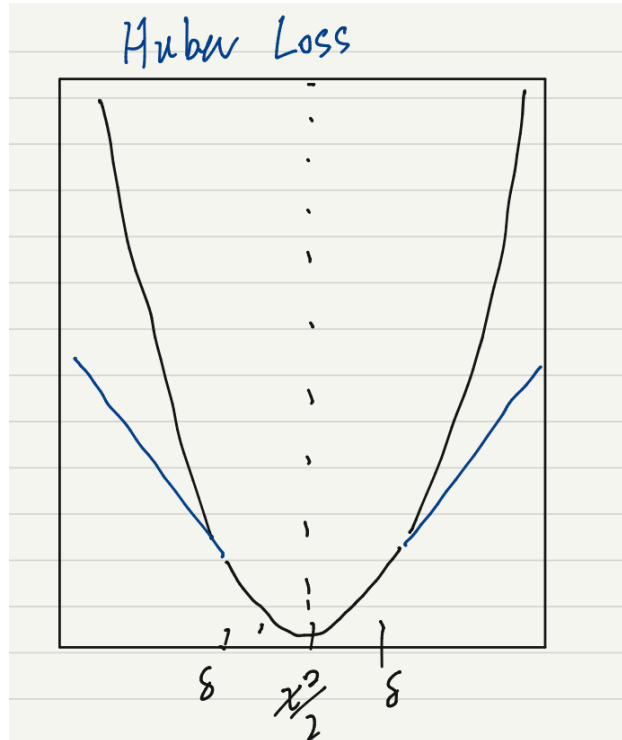
FIGURE 2. Illustration of the Huber Loss
