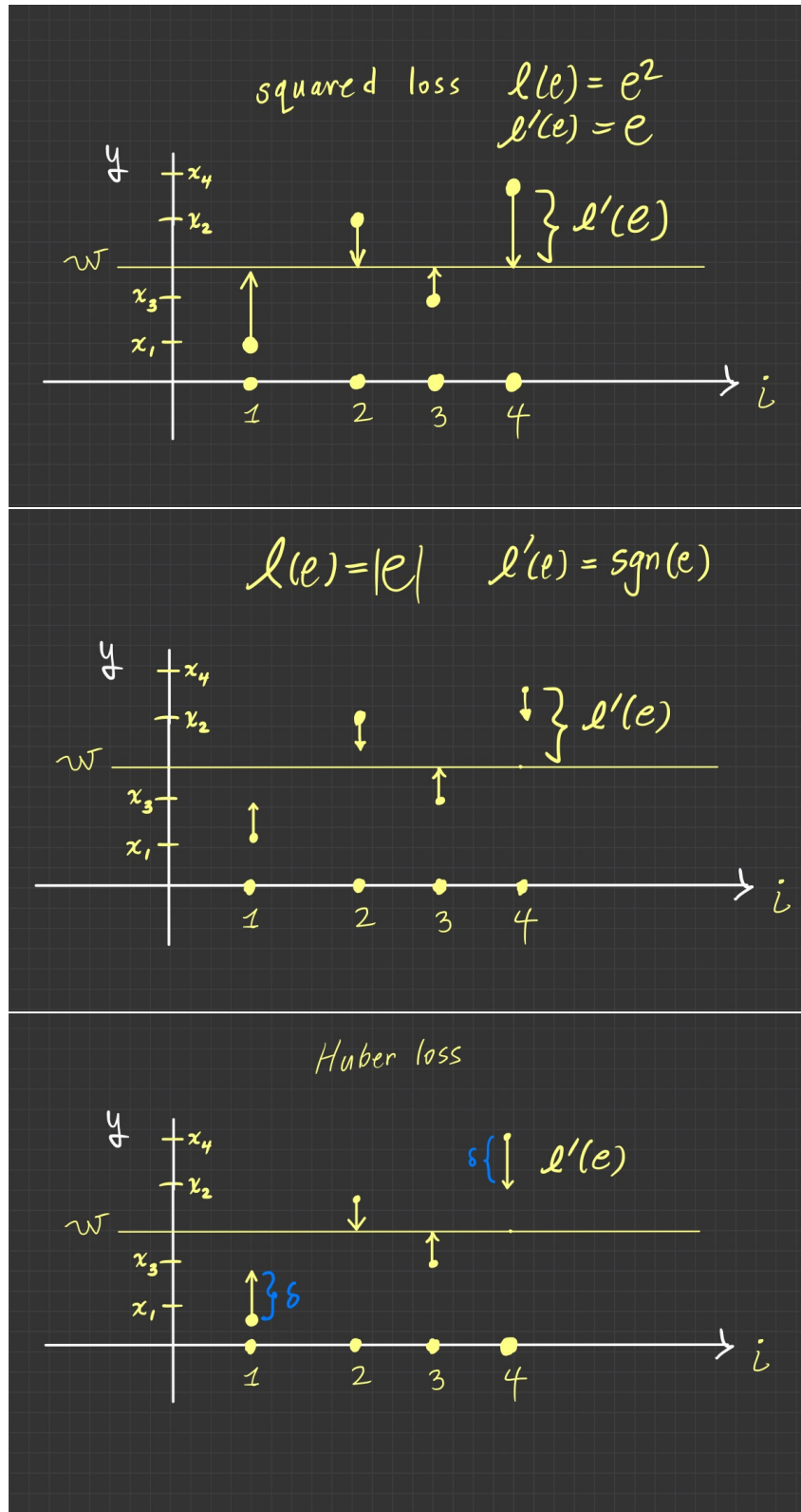
FIGURE 3. Derivative of the loss at e_i = w - x_i , for i = 1, \dots, 4 . Comparison of the quadratic, absolute, and Huber losses. The quadratic loss derivative is of size e . The absolute loss derivative is \pm 1 , the Huber loss is a combination of the two: e when |e| \leq \delta , and \pm \delta otherwise.
